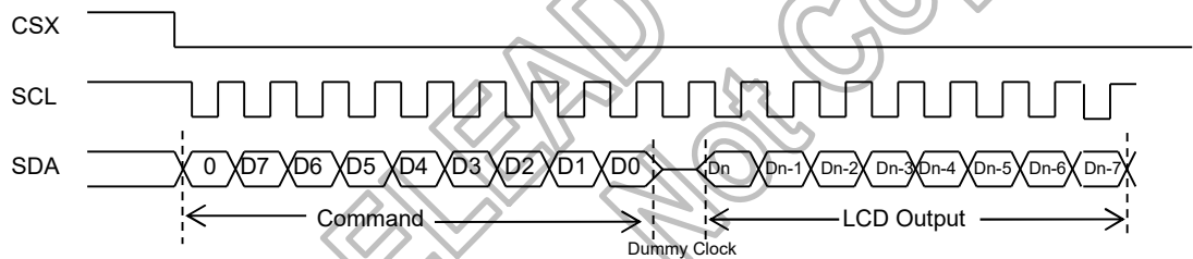
DBI Type C interface Option1: Read Over 8bits
