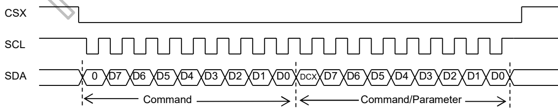
DBI Type C interface Option1
