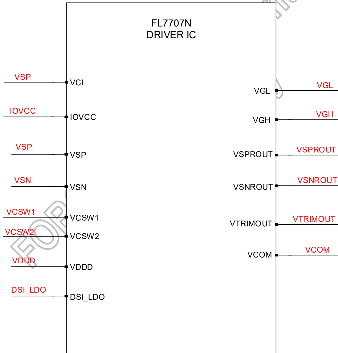
Figure 8-5: Using Three Power Mode Application
