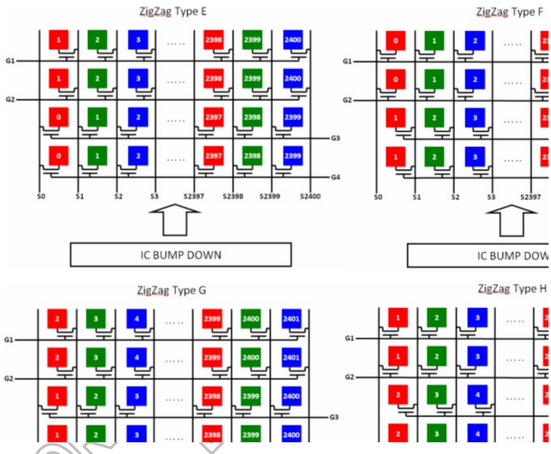
Figure 5-27: Source channels of ZigZag inversion mode
