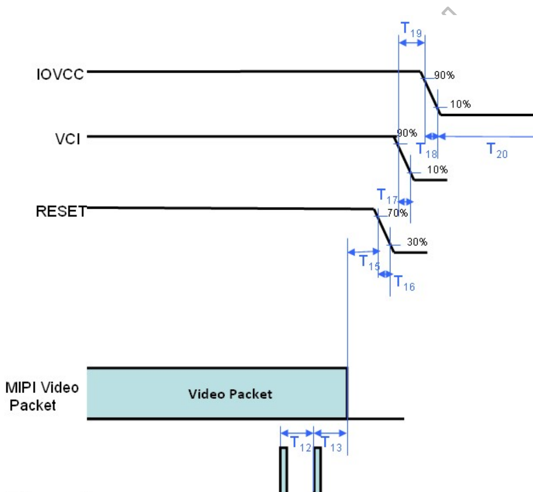
Figure 8-7: DSI Power Off Sequence of Power IC Mode
